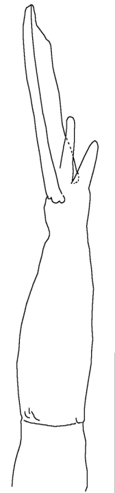
Fig. 7. Macronyssus ellipticus , male, chelicera (from Radovsky 1967). Scale bar 50 \mu m.
